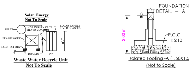
FOUNDATION DETAIL - A
