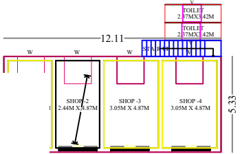
GROUND FLOOR
