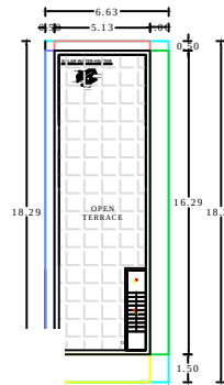
Open Terrace
