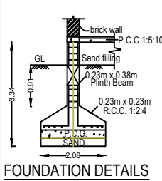
FOUNDATION DETAILS
