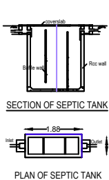
PLAN OF SEPTIC TANK
