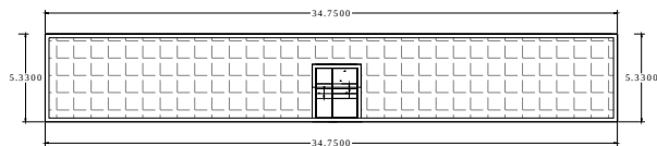
Open Terrace
