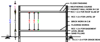
SECTION ON AA
