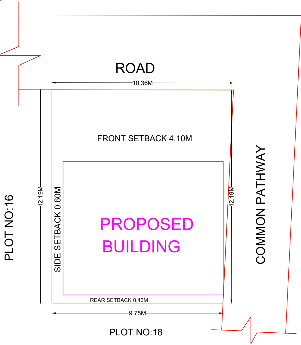
SITE PLAN
