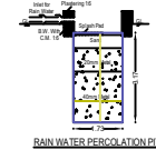
RAIN WATER PERCOLATION PIT
