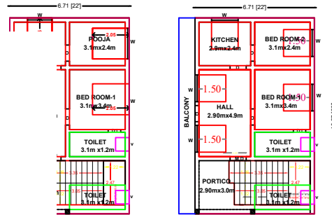
PROP.FIRST FLOOR PLAN
