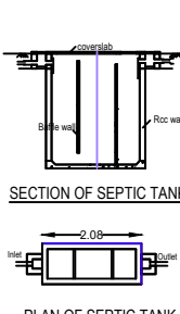
PLAN OF SEPTIC TANK
