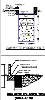
RAIN WATER COLLECTION TRENCH (SCALE-1:100)
