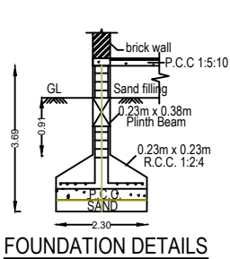
FOUNDATION DETAILS
