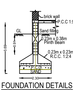
FOUNDATION DETAILS
