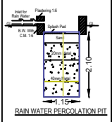
RAIN WATER PERCOLATION PIT
