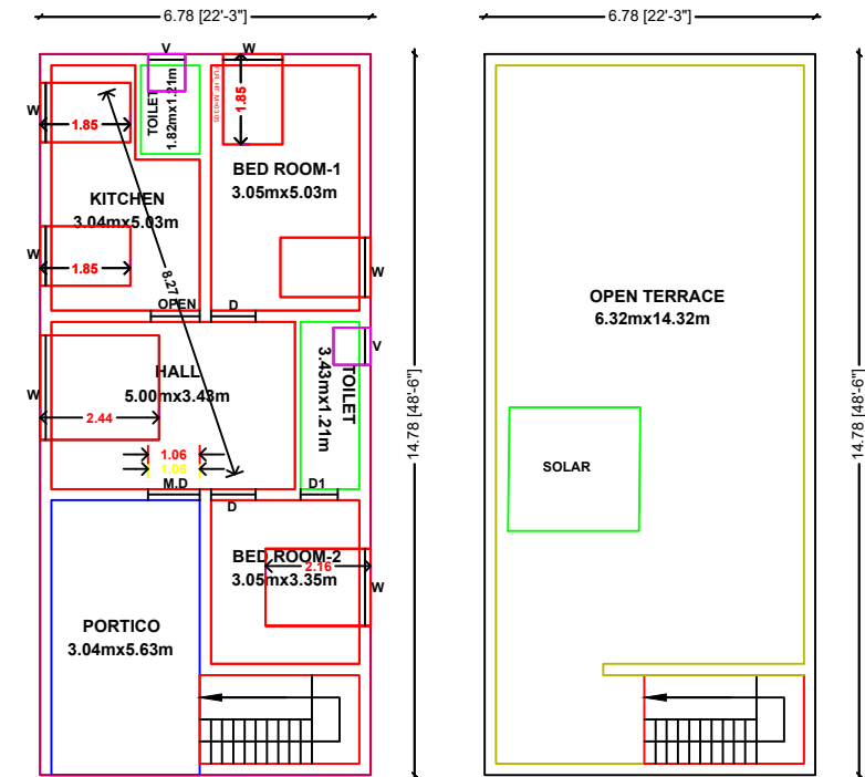
GROUND FLOOR PLAN TERRACE FLOOR PLAN
