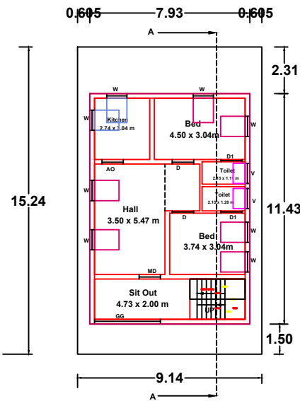
GROUND FLOOR (North Facing)
