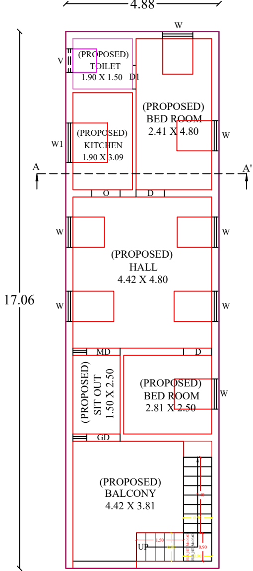
FIRST FLOOR PLAN (PROPOSED BUILDING)
