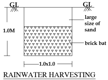
RAINWATER HARVESTING
