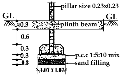
FOUNDATION DETAILS
