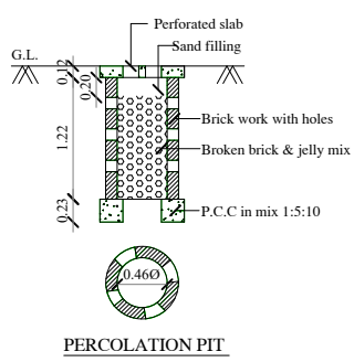
PERCOLATION PIT
