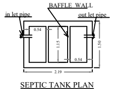
SEPTIC TANK PLAN
