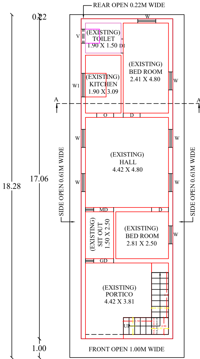
GROUND FLOOR PLAN (EXISTING BUILDING)
