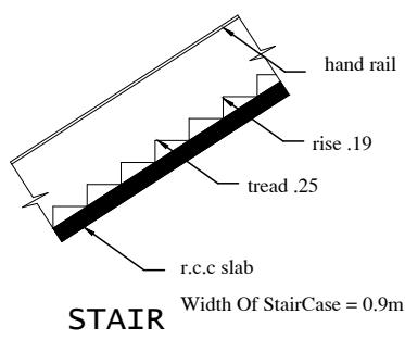
STAIR
