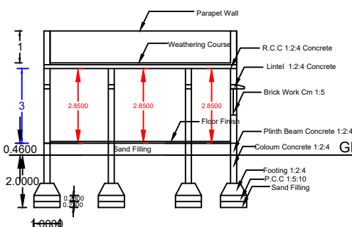
Section Section - AA
