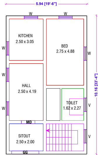
GROUND FLOOR PLAN [ NORTH FACING ]
