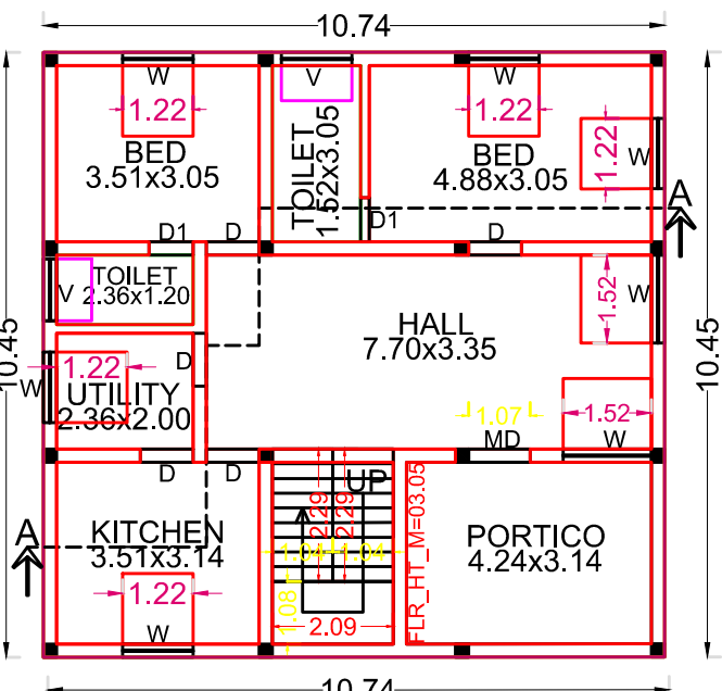
GROUND FLOOR PLAN (FACING EAST)
