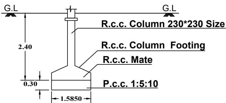
Foundation Details
