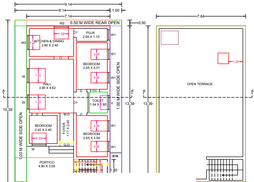
E FLOOR PLAN
