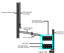
PLAN OF RAIN WATER HARVESTING
