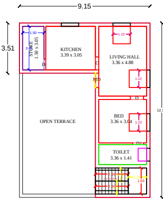
PROPOSED FIRST FLOOR PLAN EAST FACING
