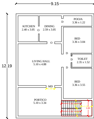
EXISTING GROUND FLOOR PLAN EAST FACING
