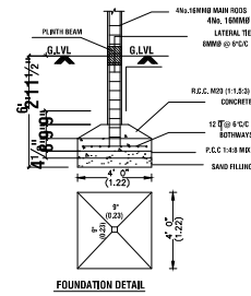
FOUNDATION DETAIL
