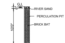
PERCOLATION PIT
