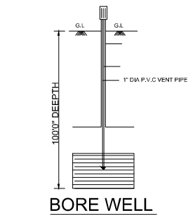
BORE WELL
