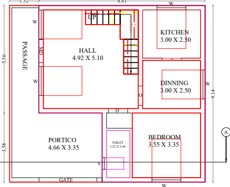
GROUND FLOOR PLAN (NORTH FACING)
