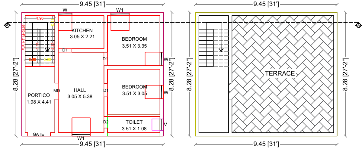
PROPOSED GROUND FLOOR PLAN TERRACE PLAN
