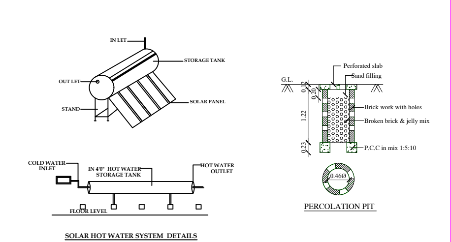
SOLAR HOT WATER SYSTEM DETAILS
