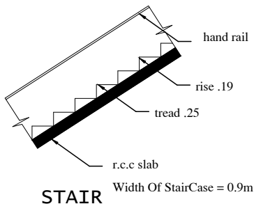
STAIR
