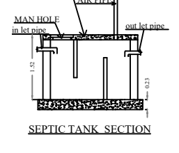
SEPTIC TANK SECTION
