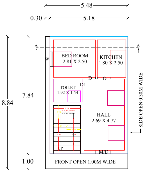
GROUND FLOOR PLAN (WEST FACING)
