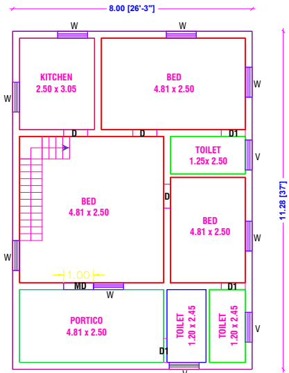
GROUND FLOOR PLAN [ WEST FACING ]
