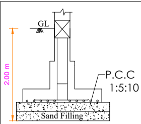
Isolated Footing - A (1.50X1.50) (Not to Scale)
