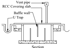
Section Plan Septic Tank With U Trap Not To Scale
