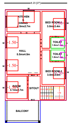
PROP.FIRST FLOOR PLAN
