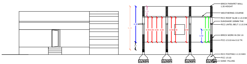
FRONT ELEVATION
