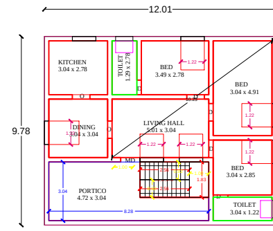
GROUND FLOOR PLAN NORTH FACING
