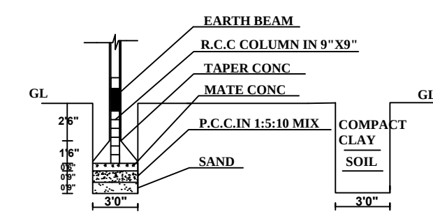
FOUNDATION DETAILS
