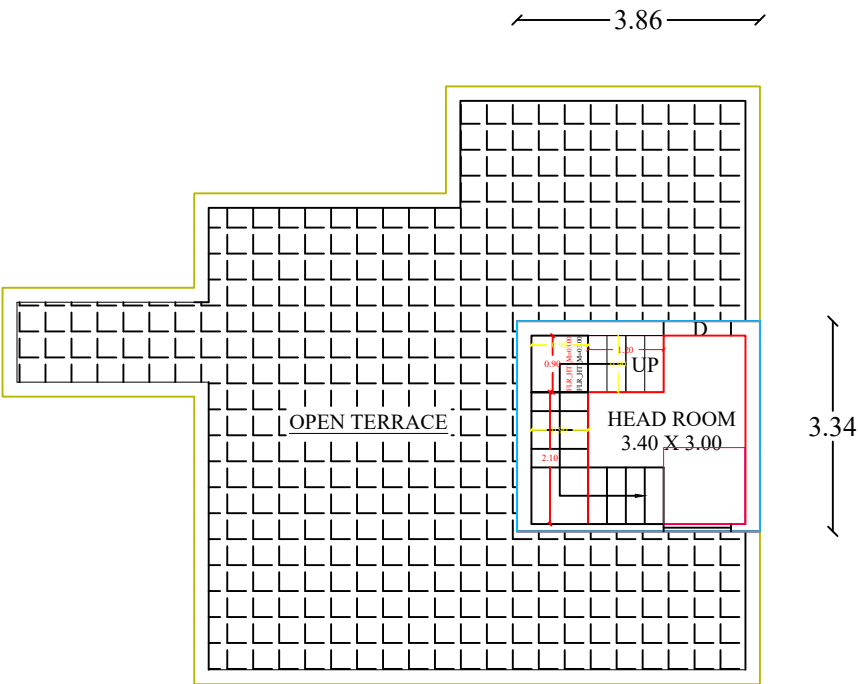
HEAD ROOM PLAN
