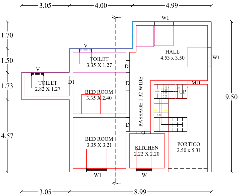
GROUND FLOOR PLAN (SOUTH FACING)
