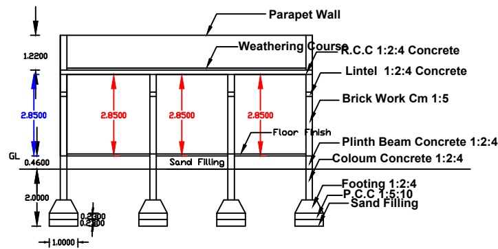
Section Section - AA
