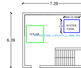
TERRACE PLAN
