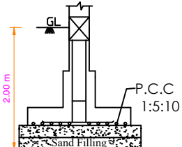
Isolated Footing - A (1.50X1.50) (Not to Scale)
