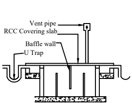
Waste Water Recycle Unit Not To Scale
