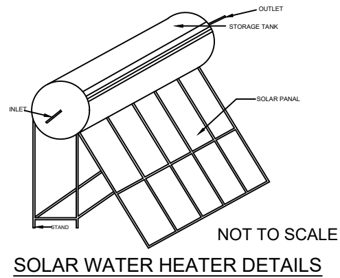
SOLAR WATER HEATER DETAILS
