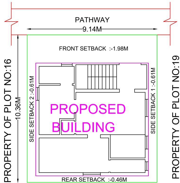
SITE PLAN
