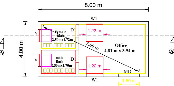
GROUND FLOOR PLAN [NORTH FACING]
