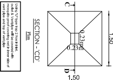
Spout Tank With U Trap
