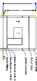
SECTION-AA
