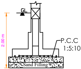
Isolated Footing -A (1.50X1.50) (Not to Scale)
