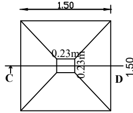
SECTION - 'CD' FOUNDATION DETAIL - A
