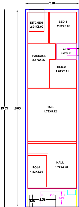
GROUND FLOOR PLAN (FACEING OF NORTH)
