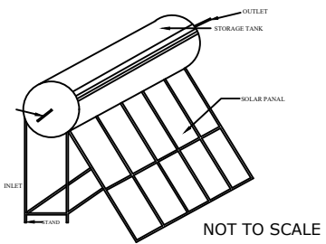
SOLAR WATER HEATER DETAILS
