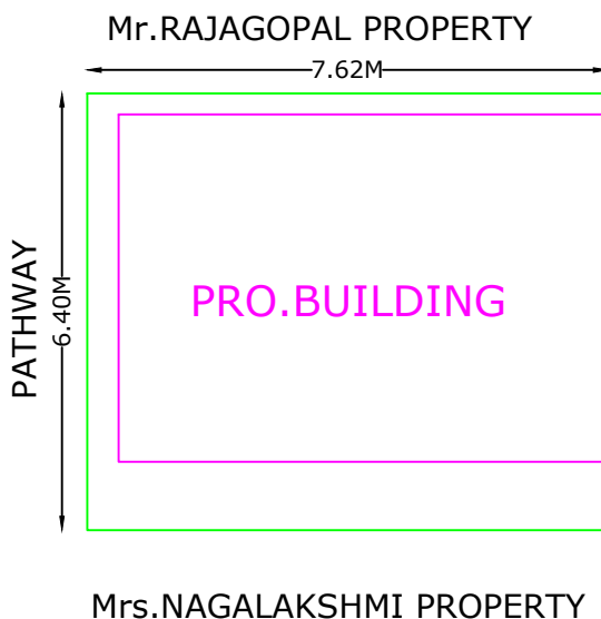
SITE PLAN
