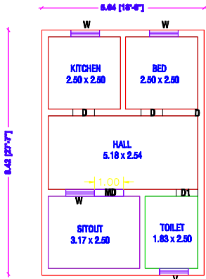
GROUND FLOOR PLAN [ NORTH FACING ]
