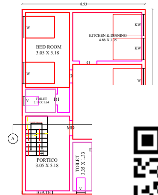
GROUND FLC (WEST FA)
