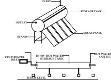
SOLAR HOT WATER SYSTEM DETAILS
