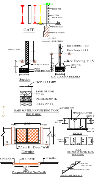
RAINWATER HARVESTING
