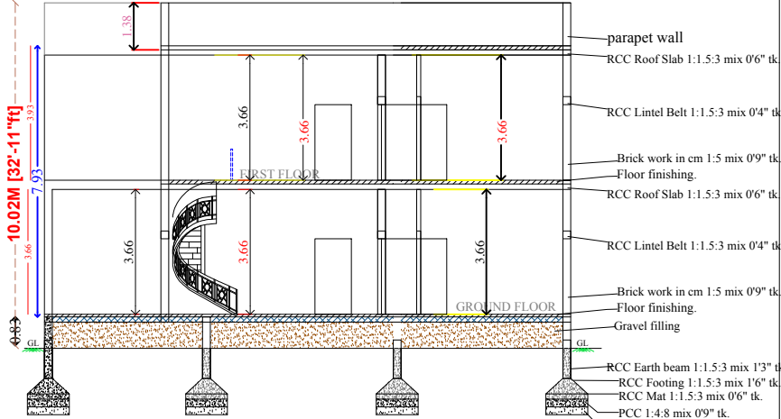
SECTIONAL DETAILS
