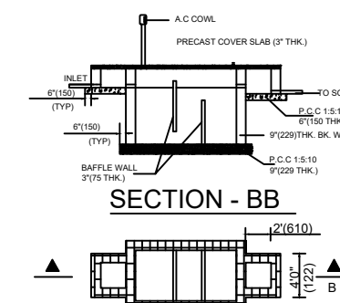
(23) (244) (23) PLAN OF SEPTIC TANK
