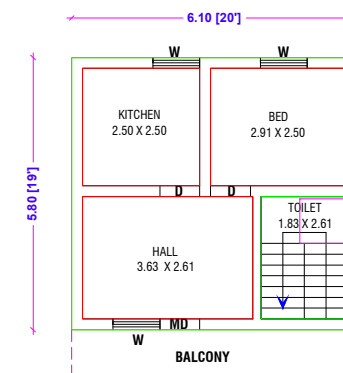
FIRST FLOOR PLAN [ NORTH FACING]
