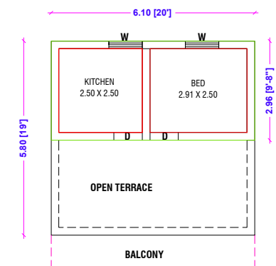
SECOND FLOOR PLAN [ NORTH FACING]
