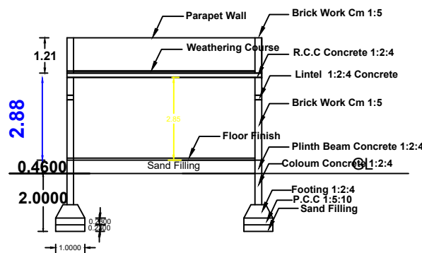
Section Section - AA
