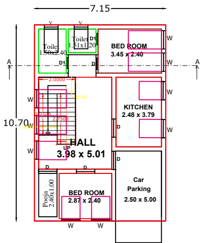
EXISTING GROUND FLOOR PLAN ( SOUTH FACING)
