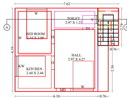
GROUND FLOOR PLAN (EAST FACING)
