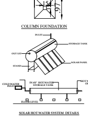
SOLAR HOT WATER SYSTEM DETAILS
