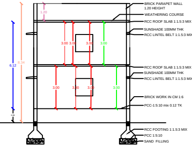
SECTION ON-AA
