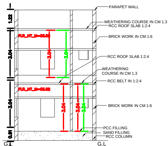
SECTION ON-AA&BB
