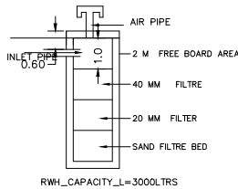
RWH_CAPACITY_L=3000LTRS
