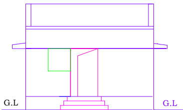
FRONT ELEVATION
