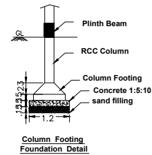
Column Footing Foundation Detail
